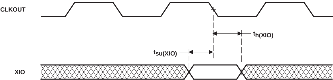
Figure 23. XIO Timing
